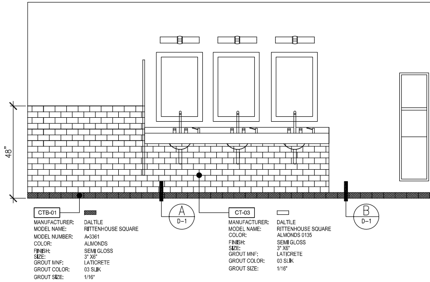
1 MEN'S RESTROOM ELEVATION SCALE 3/8" = 1' - 0"
